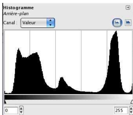
Histogramme C
