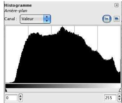
Histogramme B
