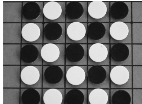
Pions
