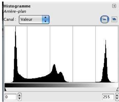
Histogramme A
